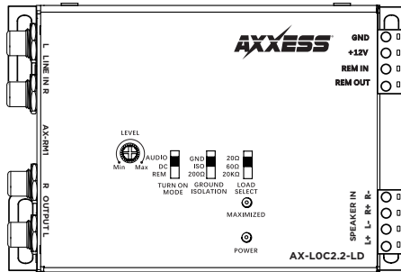
AX-LOC2.2-LD Line Out Converter (LOC)
