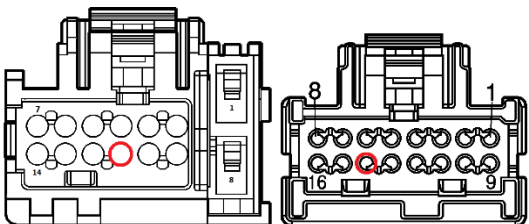
This is the pin view of the radio connectors in the vehicle
